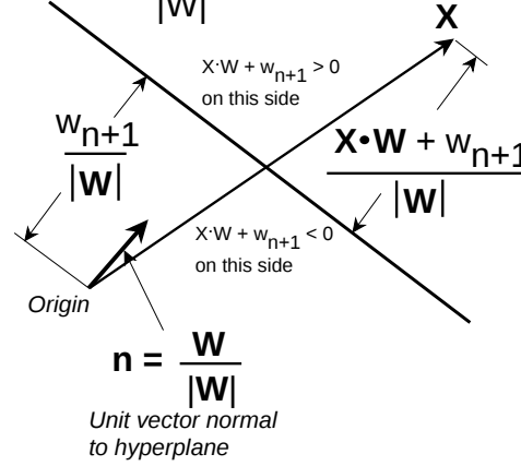
Figure 4.2: TLU Geometry
