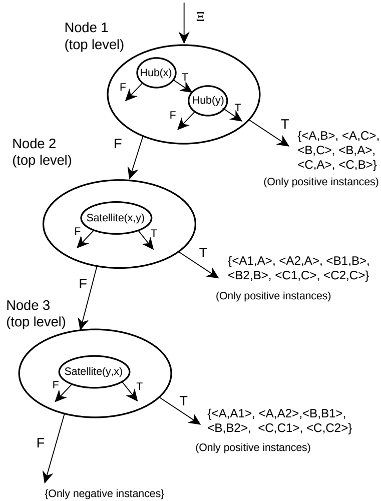
Figure 7.6: A Decision Tree for the Airline Route Problem
