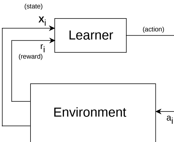
Figure 11.1: Reinforcement Learning
