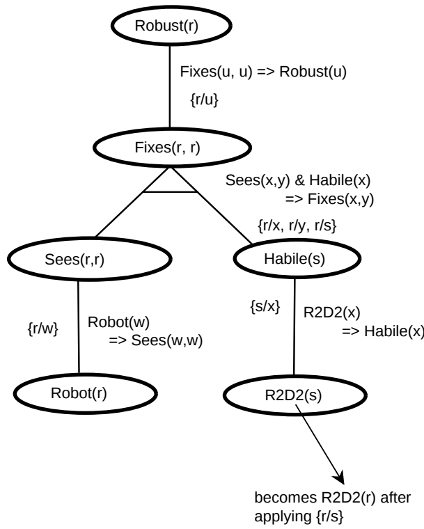
Figure 12.3: A Generalized Proof Tree
