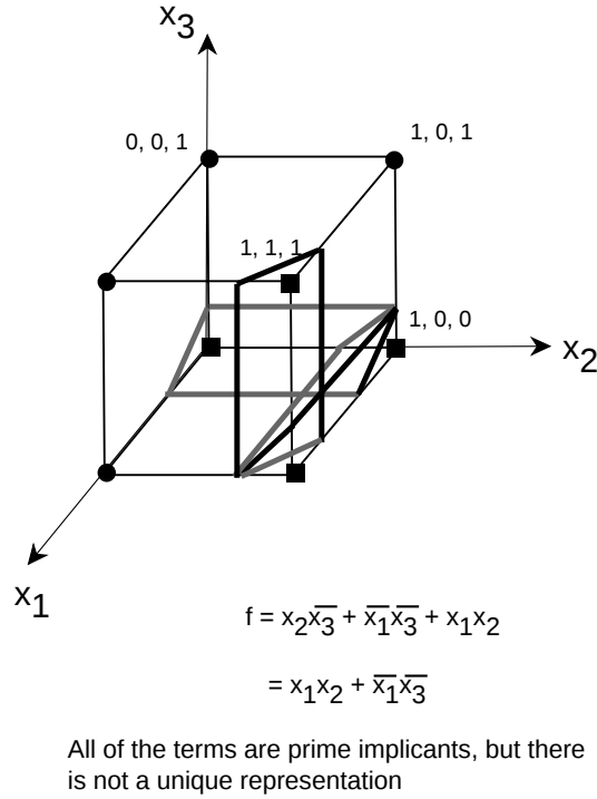
Figure 2.4: Non-Uniqueness of Representation by Prime Implicants
